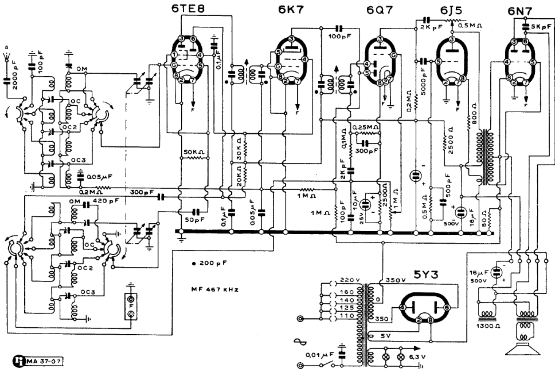
VARA RADIO - Mod. 666
